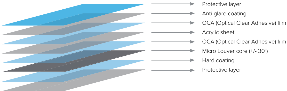
The layer construction of a Gearlab® Framed Privacy Filter.
