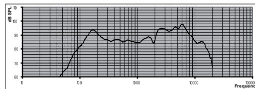
Frequency-response LC3-UC06E
