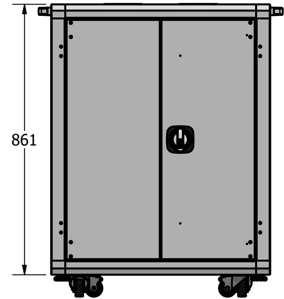
Rear View
