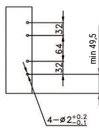
Panel frontal/ Front panel Verbox 166mm.
