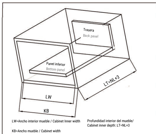
Panel frontal/ Front panel Verbox 84mm.
