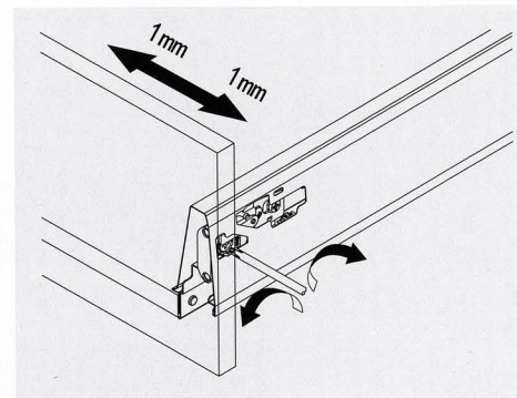
Left&right adjustment
