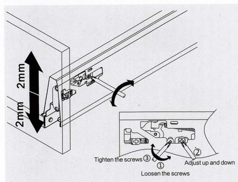
Up&down adjustment
