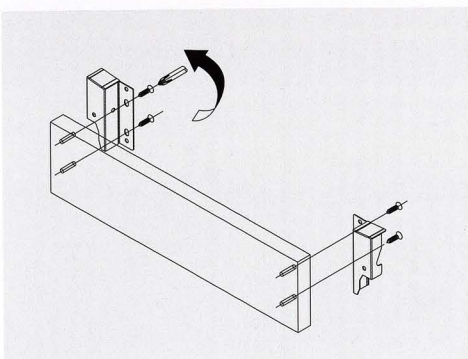
Back assembly
