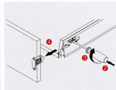
Turn screw driver to release the drawer
